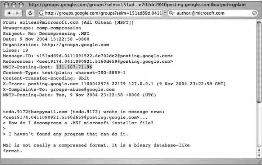
Figure 5.8 Author Search Reveals Network Traces
