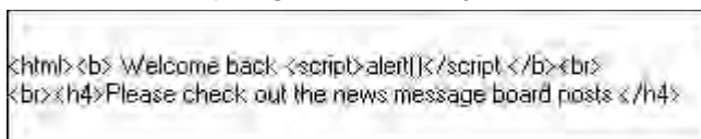
Figure B.19 Cross-Site Scripting Vulnerability in the HTTP Response
