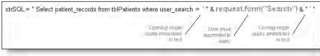
Figure B.35 A Typical SQL Query
